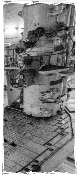
REFUELLING CRANE OF REACTOR #3
